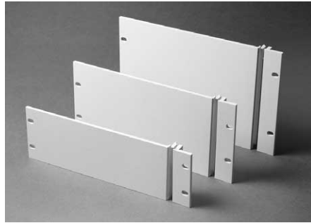
Rackmount adapter kits for 88.1 mm instrument module height (5063-9239, 5063-9240, 5063-9241)
