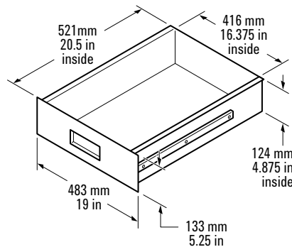
35181M Drawer
