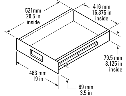
35181J Drawer
