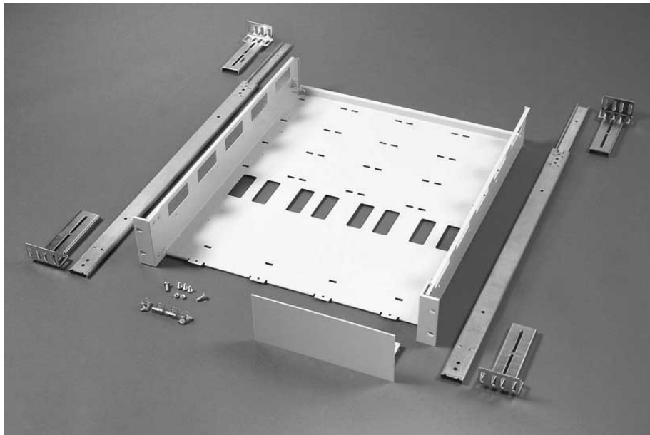
Support shelf (5063-9257), slide kit (1494-0015), and filler panel (5002-3999)
