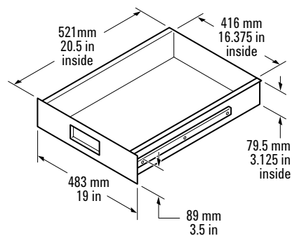
35181J Drawer
