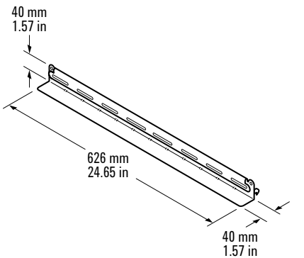
Basic rail kit (E3663AC)
